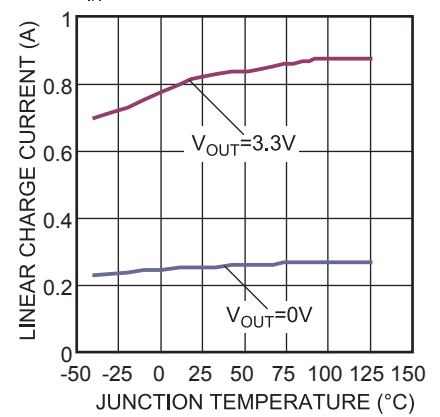
Linear Charge Current vs. Junction Temperature V_{IN}=4.2V
